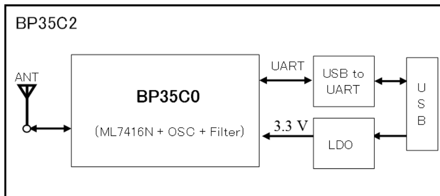
Fig. 1. Block Diagram
